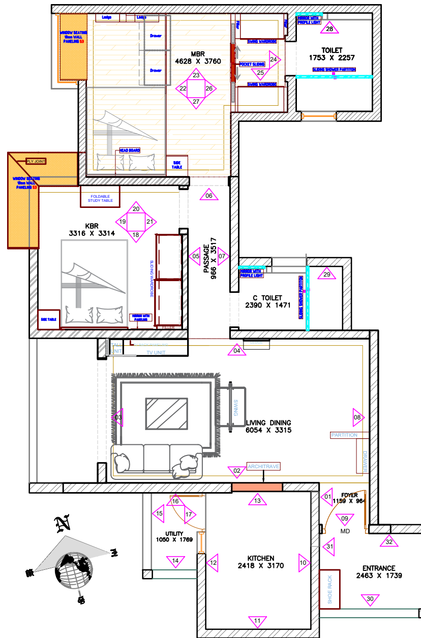
FLOOR PLAN
